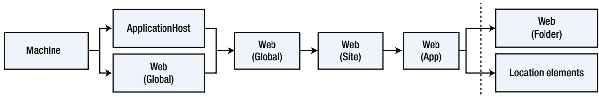
Figure 9-2. The hierarchy of ASP.NET configuration files
