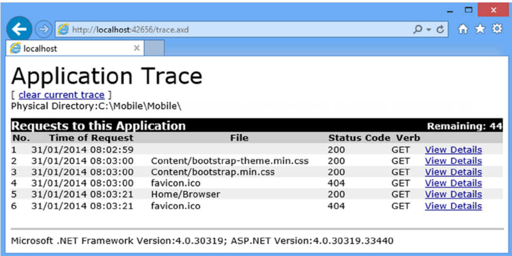
Figure 8-1. The summary of request traces
