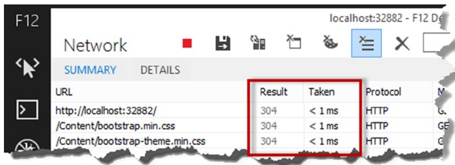
Figure 12-3. Caching content in the browser
