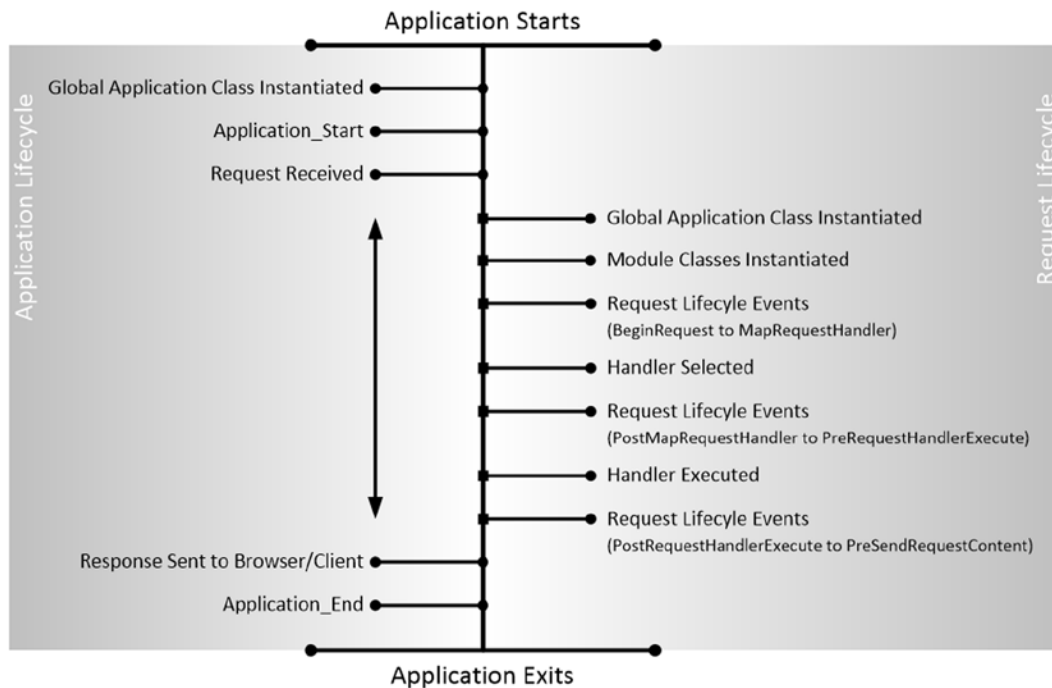
Figure 3-5. Adding the request handling process to the life-cycle diagram
