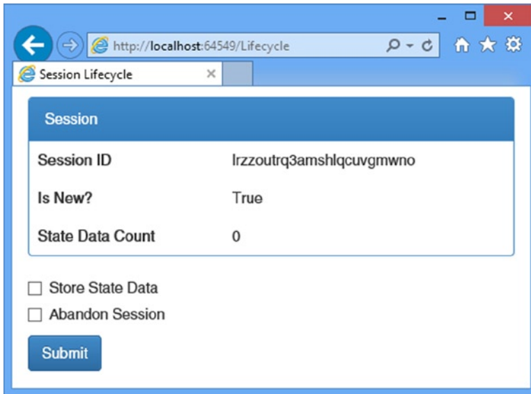
Figure 10-8. Querying and manipulating sessions
